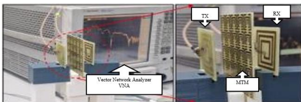
Fig. 7. Experimental setup with Modified SSRR
