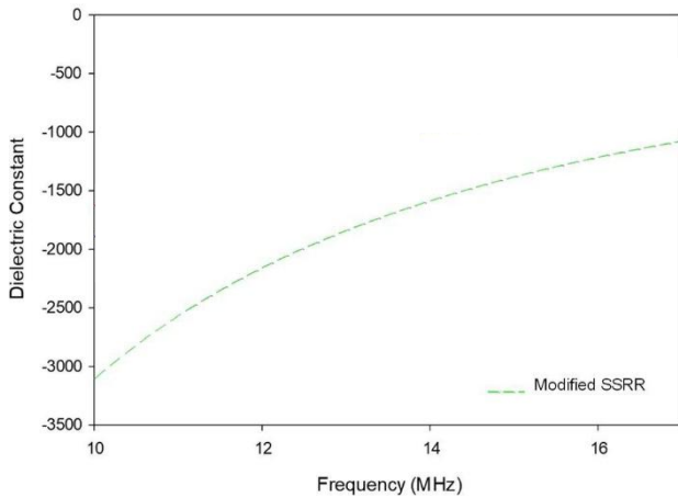
Fig. 3. Dielectric of Modified SSRR
