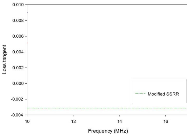
Fig. 4. Loss tangent of Modified SSRR
