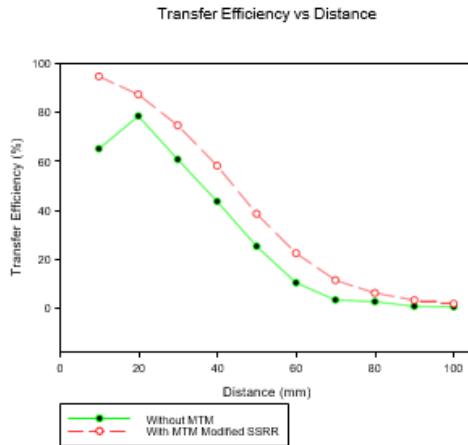
Fig. 6. Transfer Efficiency against Distance of Modified SSRR
