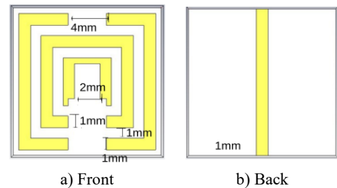
Fig. 2. MTM of Modified SSRR
