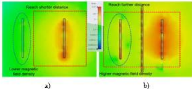
Fig. 10. Magnetic field of (a) WPT system without MTM and (b) WPT system with MTM
