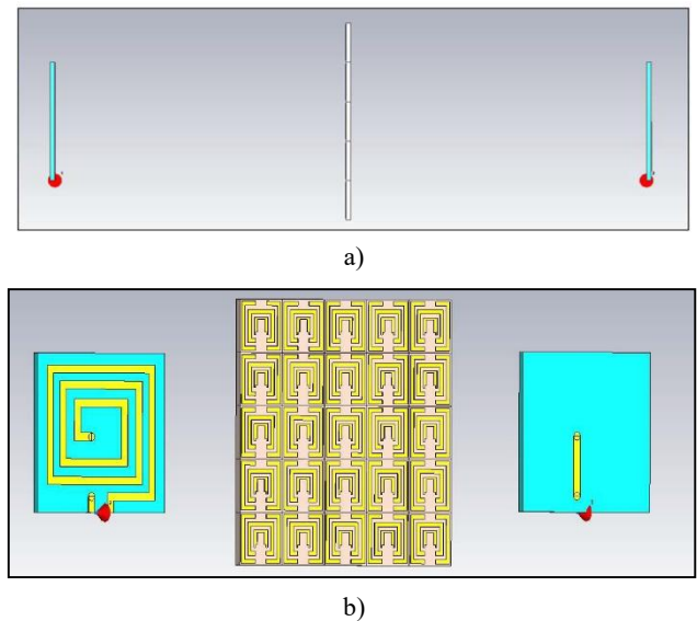
Fig. 5. Metamaterial Modified SSRR arrange from (a) 45 degree view and (b) side view
