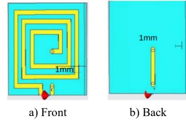
Fig. 1. Antenna for Tx and Rx
