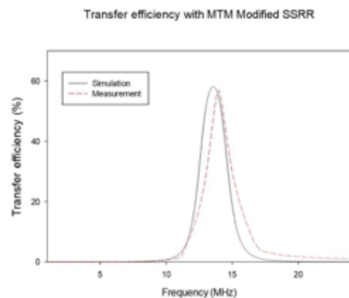
Fig. 9. Transfer Efficiency between real and simulation of with Modified SSRR
