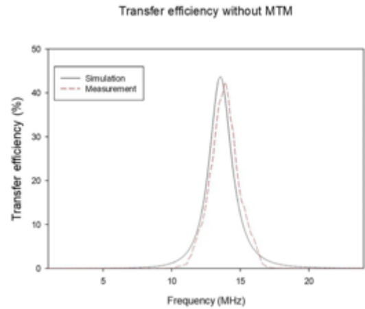
Fig. 8. Transfer Efficiency between real and simulation of without MTM
