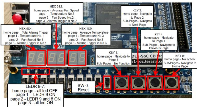
Fig. 25. FPGA Peripheral Layout for Menu Controller
