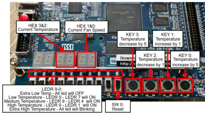
Fig. 23. FPGA Peripheral Layout for Temperature Monitor with Fan Speed Control System
