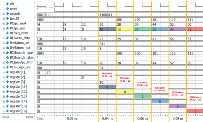
Fig. 11. Simulation Waveform for Branch Taken Cases of Branch Instructions
