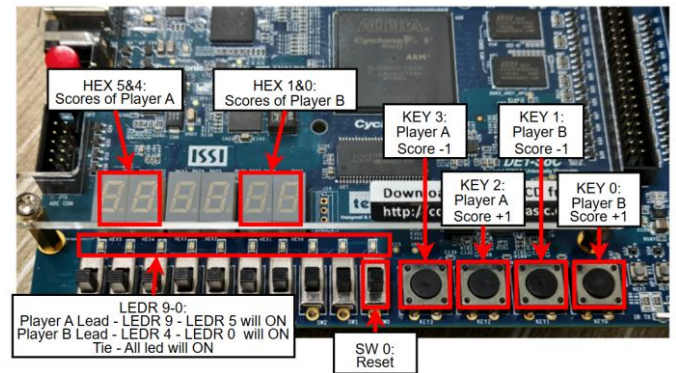
Fig. 21. FPGA Peripheral Layout for Game Score Ranking System
