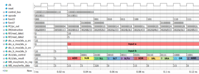
Fig. 6. Simulation Waveform for R-Type Instructions
