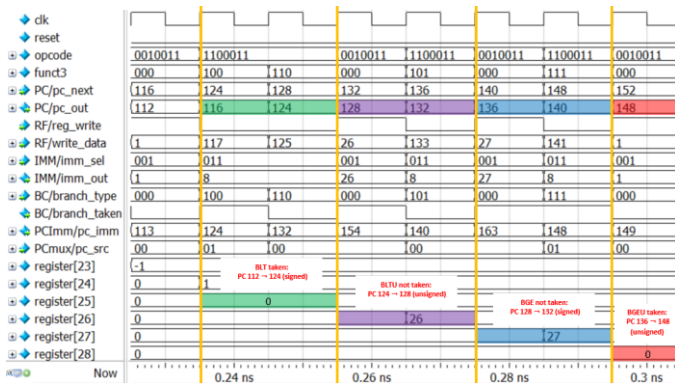
Fig. 13. Simulation Waveform for Signed and Unsigned Cases of Branch Instructions
