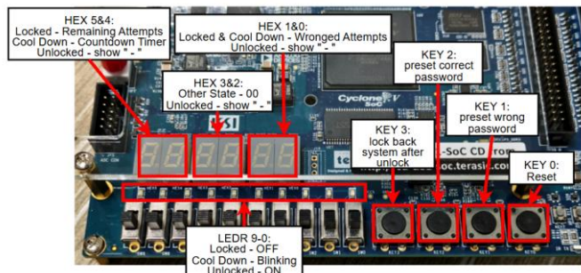
Fig. 17. FPGA Peripheral Layout for Password Lock Security System
