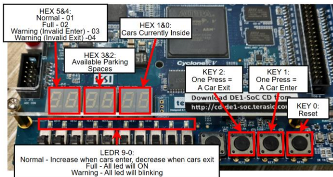
Fig. 19. FPGA Peripheral Layout for Parking Lot Management System Demonstration
