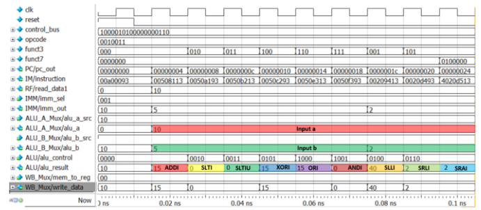
Fig. 8. Simulation Waveform for I-Type Instructions
