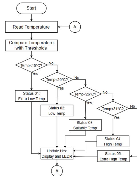
Fig. 22. Flowchart of Temperature Monitor with Fan Speed Control System
