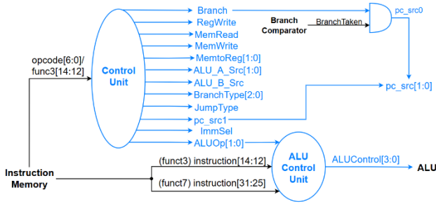
Fig. 2. The processor Control Unit and ALU Control Unit Architecture
