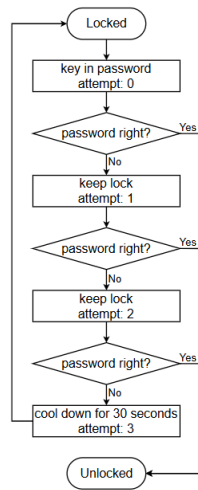
Fig. 16. Flowchart of FPGA Password Lock Security System
