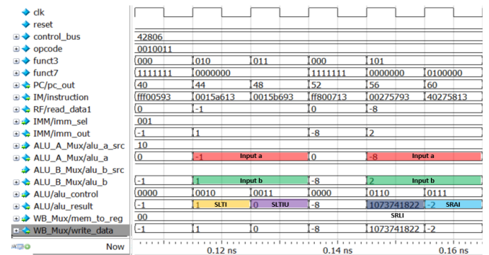
Fig. 9. Simulation Waveform for Signed and Unsigned Cases of I-Type Instructions
