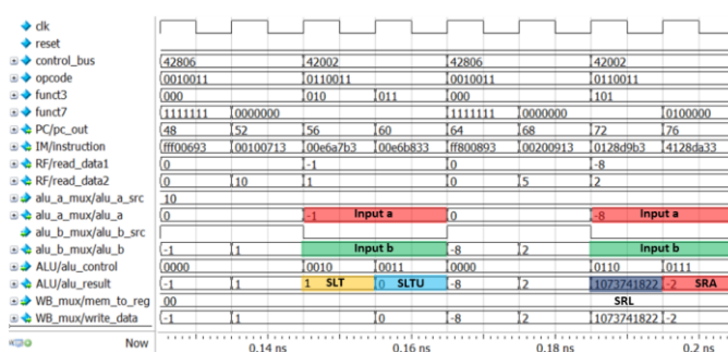
Fig. 7. Simulation Waveform for Signed and Unsigned Cases of R-Type Instructions
