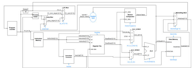
Fig. 1. The processor Datapath Architecture
