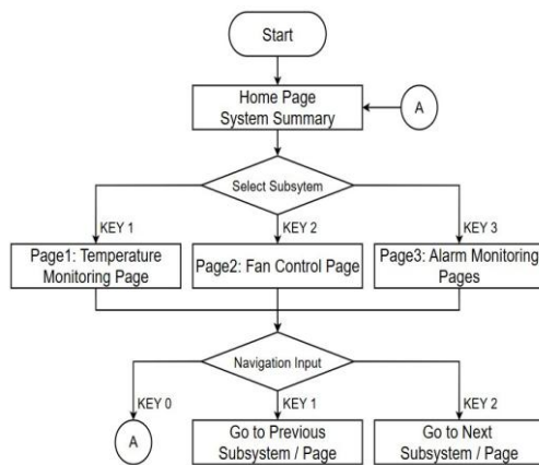
Fig. 24. Flowchart of FPGA Menu Controller
