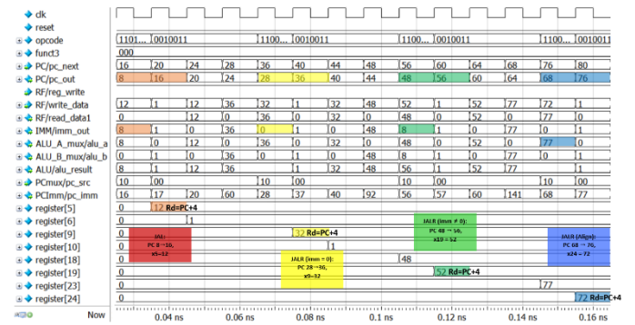
Fig. 14. Simulation Waveform for Jump Instructions
