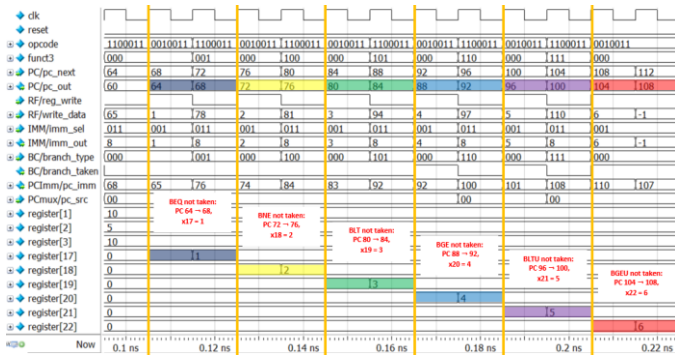
Fig. 12. Simulation Waveform for Branch Not Taken Cases of Branch Instructions
