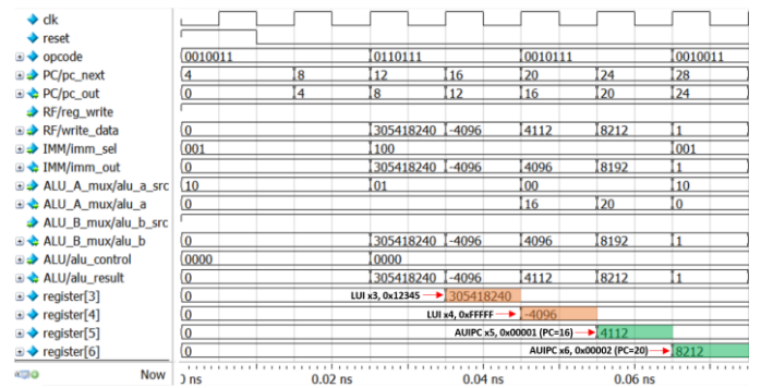
Fig. 15. Simulation Waveform for Upper Immediate Instructions
