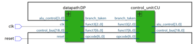
Fig. 3. Top-Level RTL for the 32-bit RISC-V Processor
