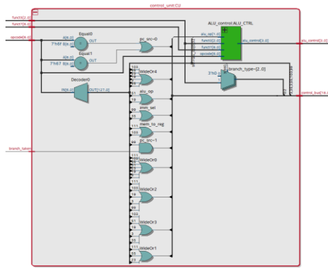
Fig. 5. RTL Representation of the Control Unit
