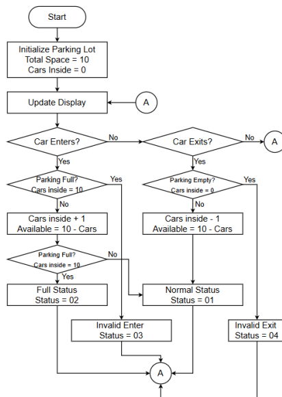
Fig. 18. Flowchart of FPGA Parking Lot Management System
